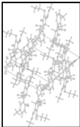
Fig. 2. The overview of I crystal packing. Atoms are represented by spheres.
