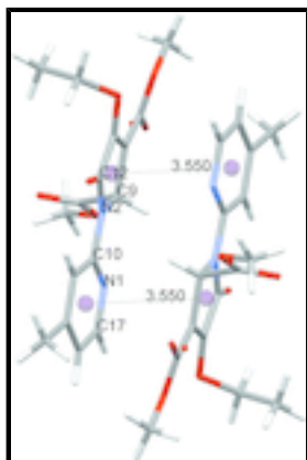
Fig. 3. Representation of \pi - \pi stacking in I.
